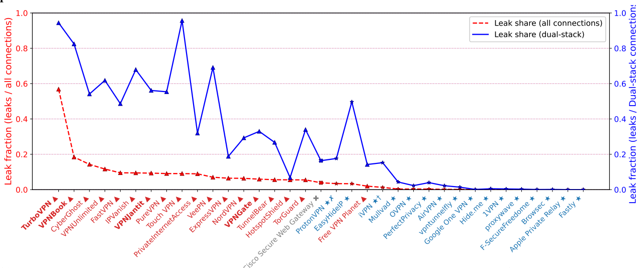
(c) Fraction of WhatIsMyIPAddress.com sessions with IPv6 leaks, shown relative to all sessions (the lower, red, dashed line) and dual-stack sessions (the upper, dark blue, solid line).
