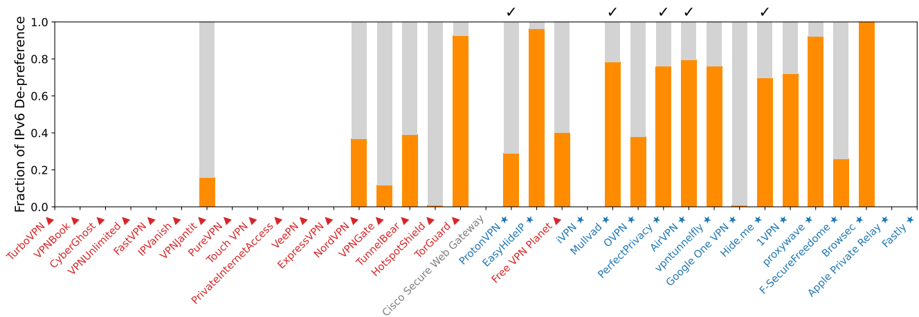
Figure 2: Fraction of dual-stack, safe, VPNs sessions to WhatIsMyIPAddress.com that de-preference IPv6 for VPNs with at least 20 such sessions per day. VPNs marked with a check were tested in §5.3
