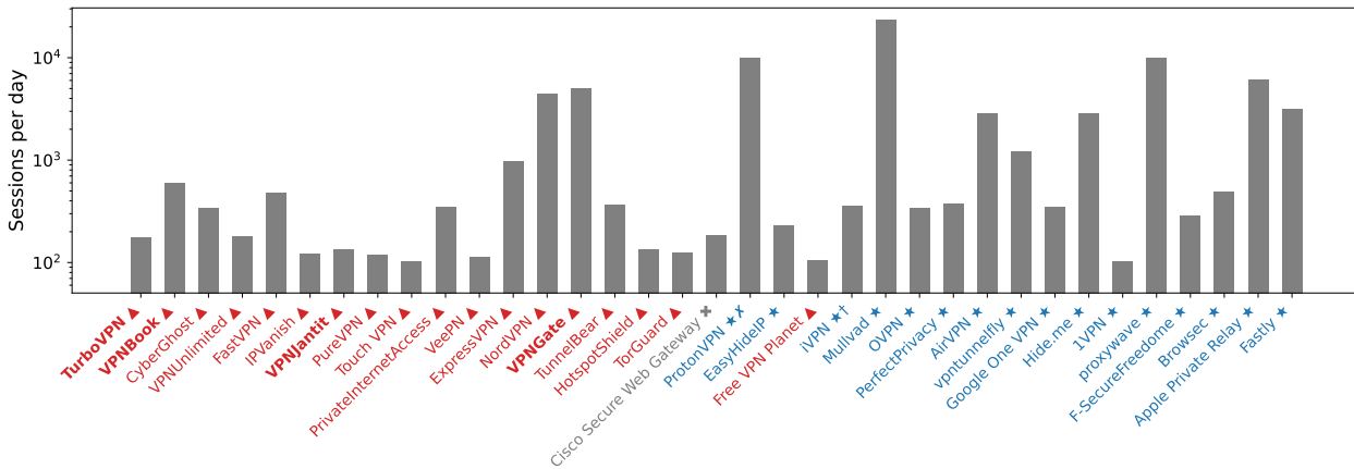
(a) Mean number of VPN sessions (log-scale) per day, for each VPN provider.
