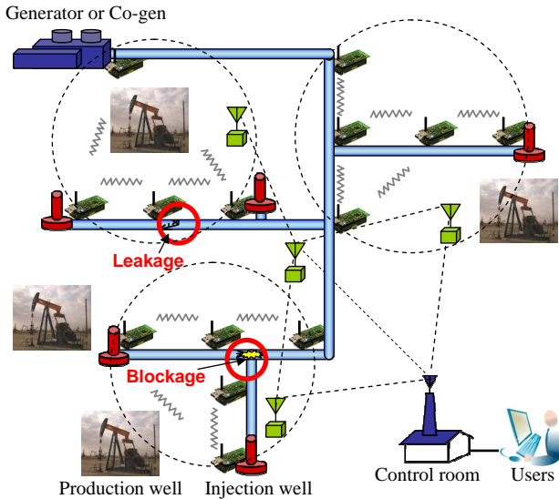
Fig. 1. A conceptual diagram of steam distribution system and monitoring it using WSN.
