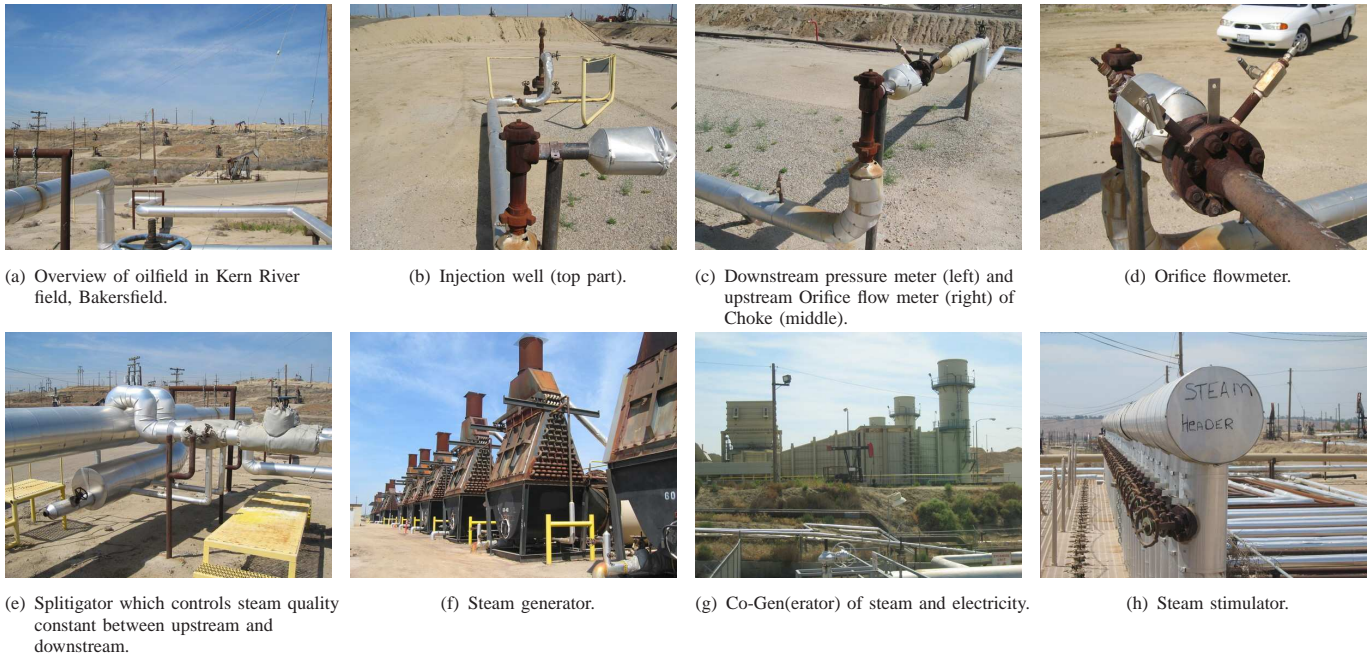
Fig. 2. Equipments currently being used in SCADA system for steamflood pipelines monitoring in oilfield.
