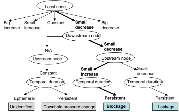
Fig. 3. An example of decision tree on pressure for blockage, leakage, and downhole pressure change.
