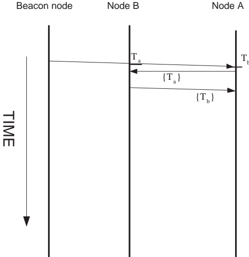
Fig. 5. Receiver-Receiver Synchronization
