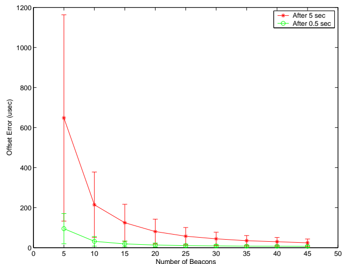
Fig. 10. Effect of Changing the Number of Sync Beacons
