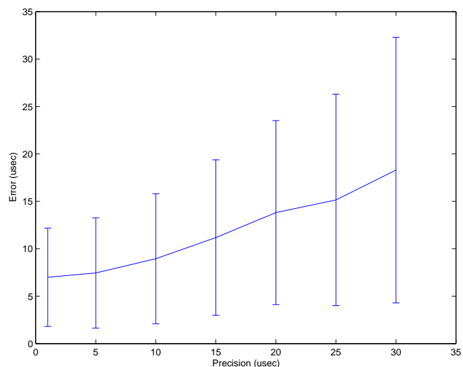
Fig. 11. Varying the Clock Granularity
