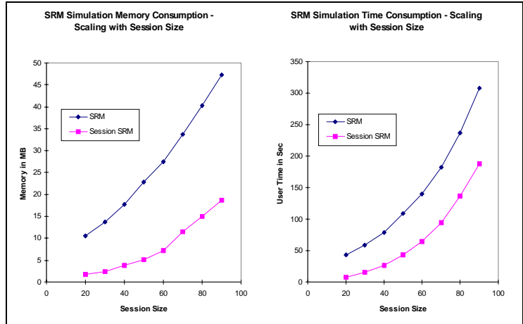
Figure 7. Performance Comparison for SRM and Session SRM
