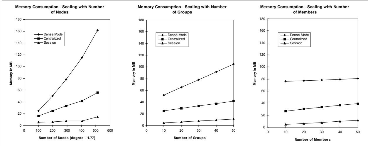
Figure 3. Comparison of Memory Usage
