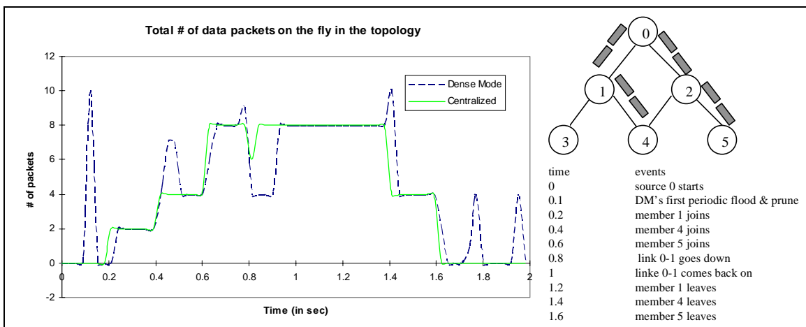
Figure 5. Difference Between Dense Mode and Centralized Multicast
