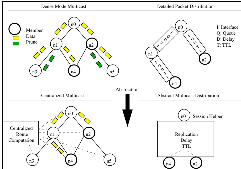
Figure 1. Illustration of the Detailed and Abstract Simulation Mechanisms
