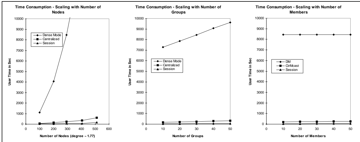
Figure 4. Comparison of Time Usage
