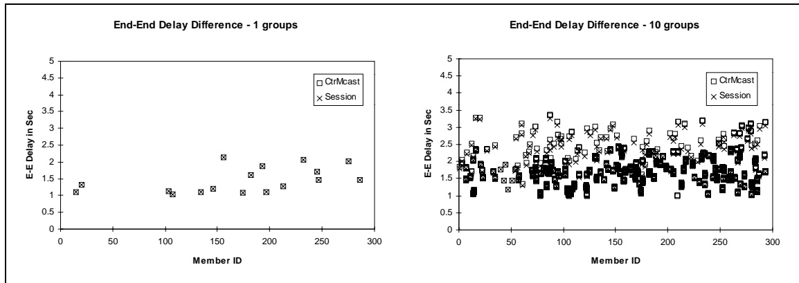
Figure 6. Difference Between Detailed Packet Distribution and Abstract Multicast Packet Distribution
