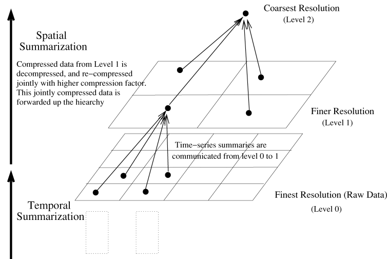
Fig. 2. Hierarchy construction.
