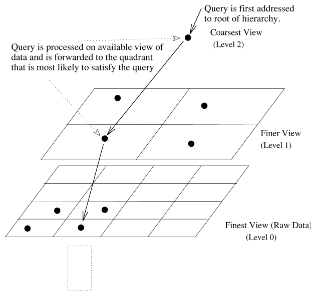
Fig. 3. Drill-down querying.
