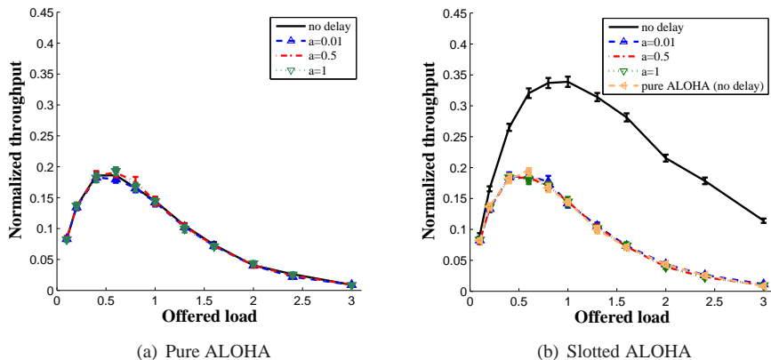
Figure 3: Throughput of pure and slotted ALOHA protocols vs. offered load (packets/transmission time); a is a parameter representing varying maximum propagations by normalizing the delay to the transmission time (more details in Section 5.1). This figure shows that for any value a > 0 , slotted ALOHA degrades to pure ALOHA in underwater networks.
