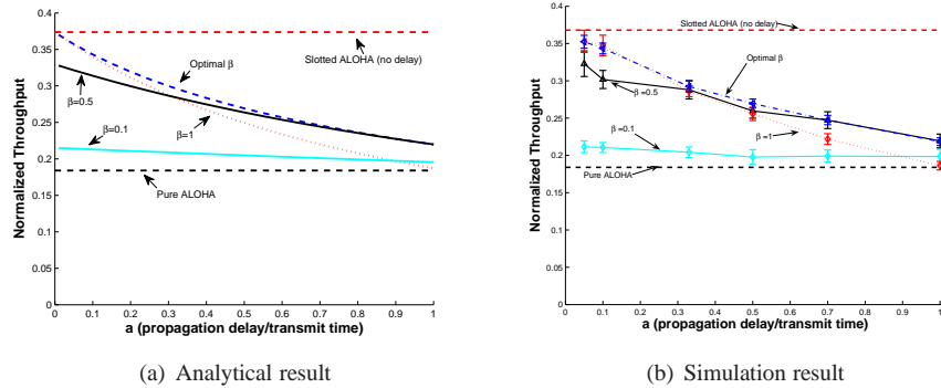
Figure 11: Maximum throughput of PDT-ALOHA as the normalized propagation delay a is varied.
