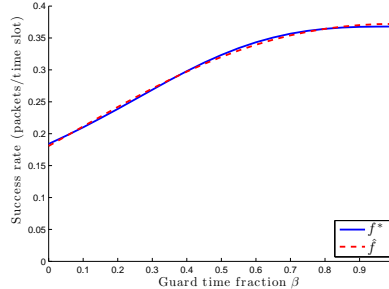
Figure 8: The maximum success rate; numerically calculated values of f^* and its approximation \hat{f}
