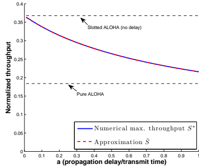
Figure 7: Maximum throughputs of PDT-ALOHA depending on the guard time size
