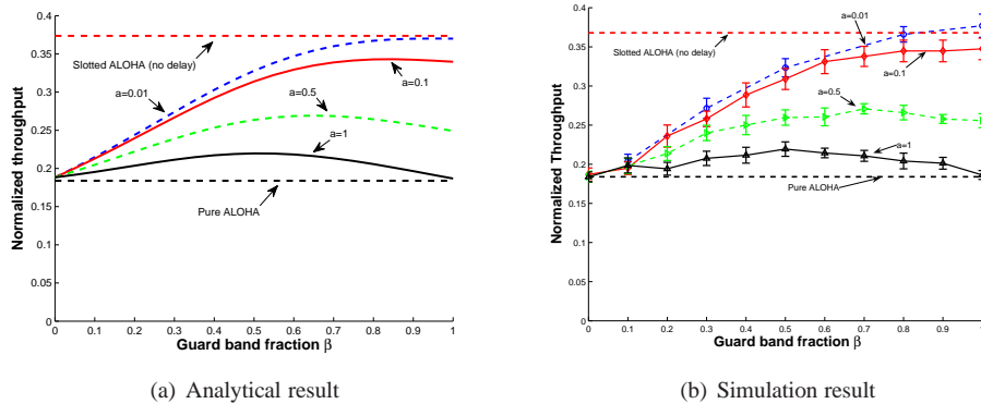
Figure 10: Throughput of PDT-ALOHA as guard time length \beta is varied.
