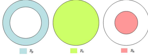
Figure 6: Collision regions: R_p is the region from which packets sent in the previous consecutive time slot would collide with the interested packet, R_c is the region for transmitters for the intra-timeslot collision, and R_n is the region for transmitters in the next time slot for the inter-timeslot collision.
