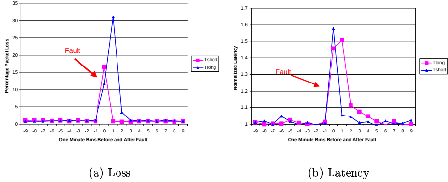
Figure 4: Average percentage end-to-end loss and normalized latency of 512 byte ICMP echos sent to 100 web sites every second during the ten minutes immediately proceeding and following the injection of a Tshort and Tlong events at the Mae-West exchange point.
