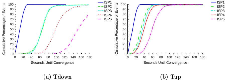
Figure 3: Convergence latency of a cumulative percentage of Tdown and Tup events injected at the Mae-West exchange point for five major ISPs
