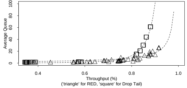
Figure 5: Comparing Drop Tail and RED gateways.
